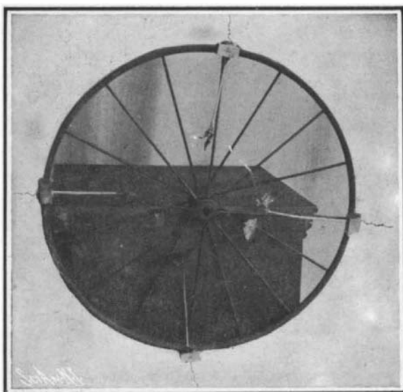
The roots grow centrifugally on a rotating wheel.
