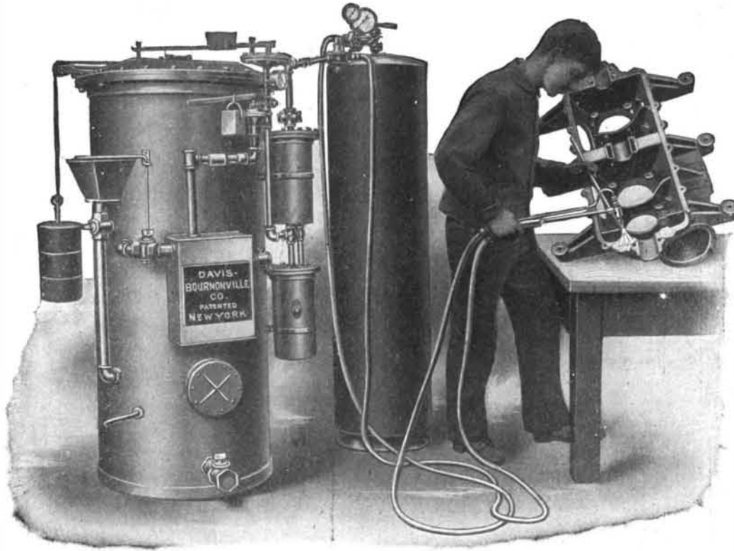
Repairing an Aluminum Automobile Gear Case
