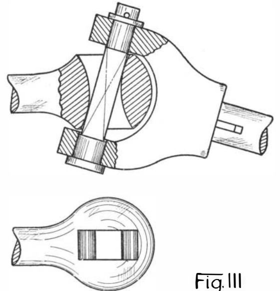
THE SQUARE PIN UNIVERSAL JOINT.
