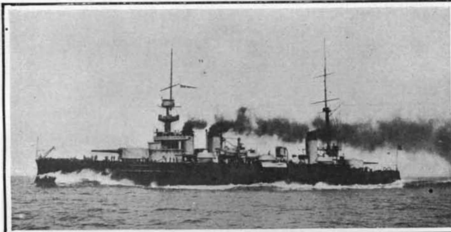
Displacement, 14,900 tons. Speed, 19.5 knots. Coal, 1,825 tons. Armor: Belt, 11 inches; deck, 3¾ inches; main turrets, 12 inches; secondary turrets, 5½ inches; casemates, 5½ inches. Guns: Four 50-caliber 12-inch; ten 7.6-inch; twenty-three small guns. Torpedo tubes, 4. Complement, 793. Battleship "Démocratie." Four Ships.
