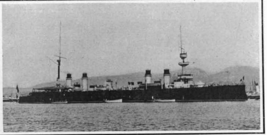
Displacement, 10,000 tons. Speed, 21.6 knots. Coal, 1,590 tons. Armor: Belt, 6¾ inches; deck, 2½ inches; main turrets, 8 inches; secondary turrets, 4¾ inches; casemates, 4¾ inches. Guns: Two 7.6-inch; eight 6.4-inch; six 4-inch; twenty small guns. Torpedo tubes, 5. Complement, 550. Armored Cruiser "Marseillaise." Four Ships.
