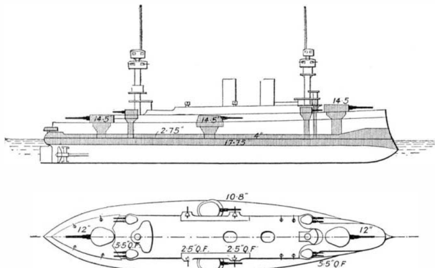
Displacement, 11,900 tons. Speed, 18 knots. Coal, 1,100 tons. Armor: Belt, 17¾ to 9¾ inches; decks, 2¾ and 1½ inches; side, 4 inches; main turrets, 14½ inches; secondary turrets, 4 inches. Armament: Two 12-inch; two 10.8-inch; eight 5.5-inch; twenty small guns. Torpedo tubes, 4. Complement, 607.
