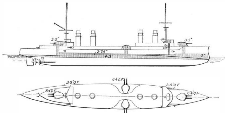
Displacement, 7,700 tons. Speed, 21 knots. Coal, 1,200 tons, plus oil. Armor: Belt, 4 to 3¼ inches; deck, 2¾ inches; turrets, 4 inches. Armament: Eight 6.4-inch; four 4-inch; ten small guns. Torpedo tubes, 2. Complement, 550.
