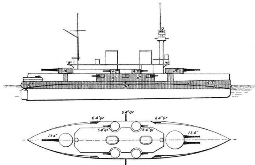
Displacement, 11,395 tons. Speed, 18 knots. Coal, 890 tons. Armor: Belt, 18 to 12 inches; deck, 3 inches; side, 4¾ inches; turrets, 18 inches; secondary turrets, 4¾ inches. Armament: Three 42-caliber 13.4-inch; ten 6.4-inch; twenty small guns. Torpedo tubes, 6. Complement, 696.
