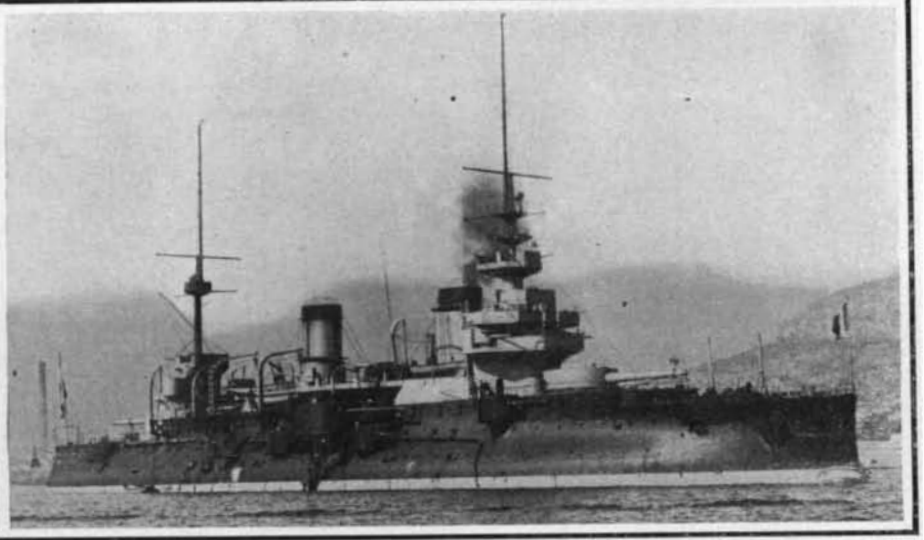
Displacement, 12,205 tons. Speed, 17½ knots. Coal, 800 tons. Armor: Belt, 16 inches; decks, 3½ and 1¾ inches; sides, 4 inches; main turrets, 14 inches; secondary turrets, 4 inches. Guns: Two 12-inch; two 10.8-inch; eight 5.5-inch; eight 4-inch; thirty small guns. Torpedo tubes, 4. Complement, 630. Battleship "Bouvet." Four Ships (Approximate).
