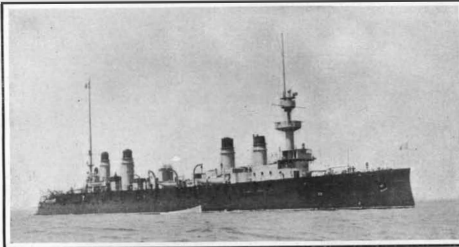
Displacement, 9,517 tons. Speed, 21.1 knots. Coal, 1,600 tons, plus oil. Armor: Belt, 6¾ inches; side, 3¾ inches; deck, 2 inches; turrets, 8 inches; casemates, 4 inches. Guns: Two 7.6-inch; eight 6.4-inch; four 4-inch. Torpedo tubes, 2. Complement, 612. Armored Cruiser "Montcalm." Three Ships.
