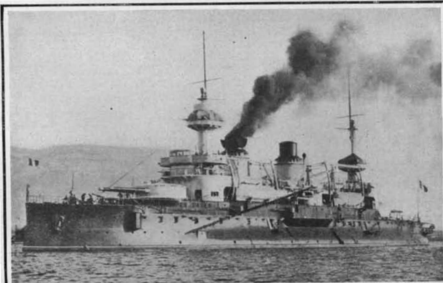
Displacement, 11,260 tons. Speed, 18.2 knots. Coal, 1,100 tons. Oil, 200 tons. Armor: Belt, 16 inches; decks, 2¾ and 1½ inches; sides, 3 inches; main turrets, 9 and 11 inches; secondary battery, 3 inches. Guns: Four 12-inch; ten 5.5-inch; eight 4-inch; twenty small guns. Torpedo tubes, 4. Complement, 631. Battleship "Gaulois." Three Ships.
