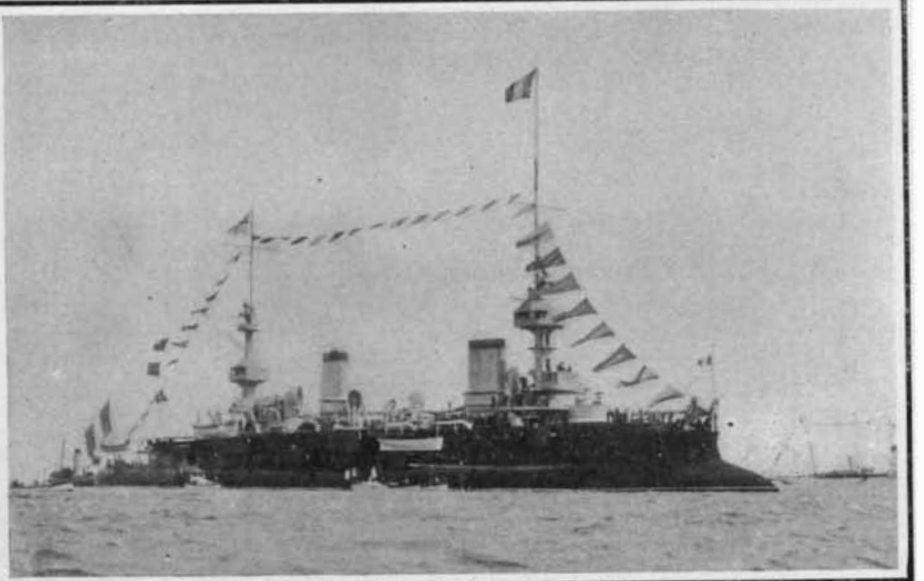
Displacement, 11,924 tons. Speed, 18 knots. Coal, 800 tons, plus oil. Armor: Belt, 17¾ inches; decks, 3½ and 1¾ inches; turrets, 16 inches; secondary turrets, 4 inches. Guns: Two 12-inch; two 10.8-inch; eight 5.5-inch; eight 4-inch; fourteen small guns. Torpedo tubes, 4. Complement, 617. Battleship "Massena."
