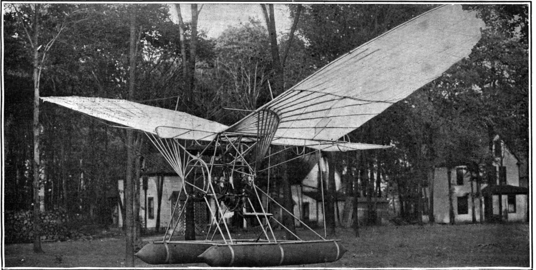
The Gammeter Orthopter. Width, 30 Feet from Tip to Tip; Length, Including Rudder, 12 Feet; Area of Body, Including Rudder, 48 Square Feet; Area of Wings, 154 Square Feet; Total Area, 202 Square Feet.
