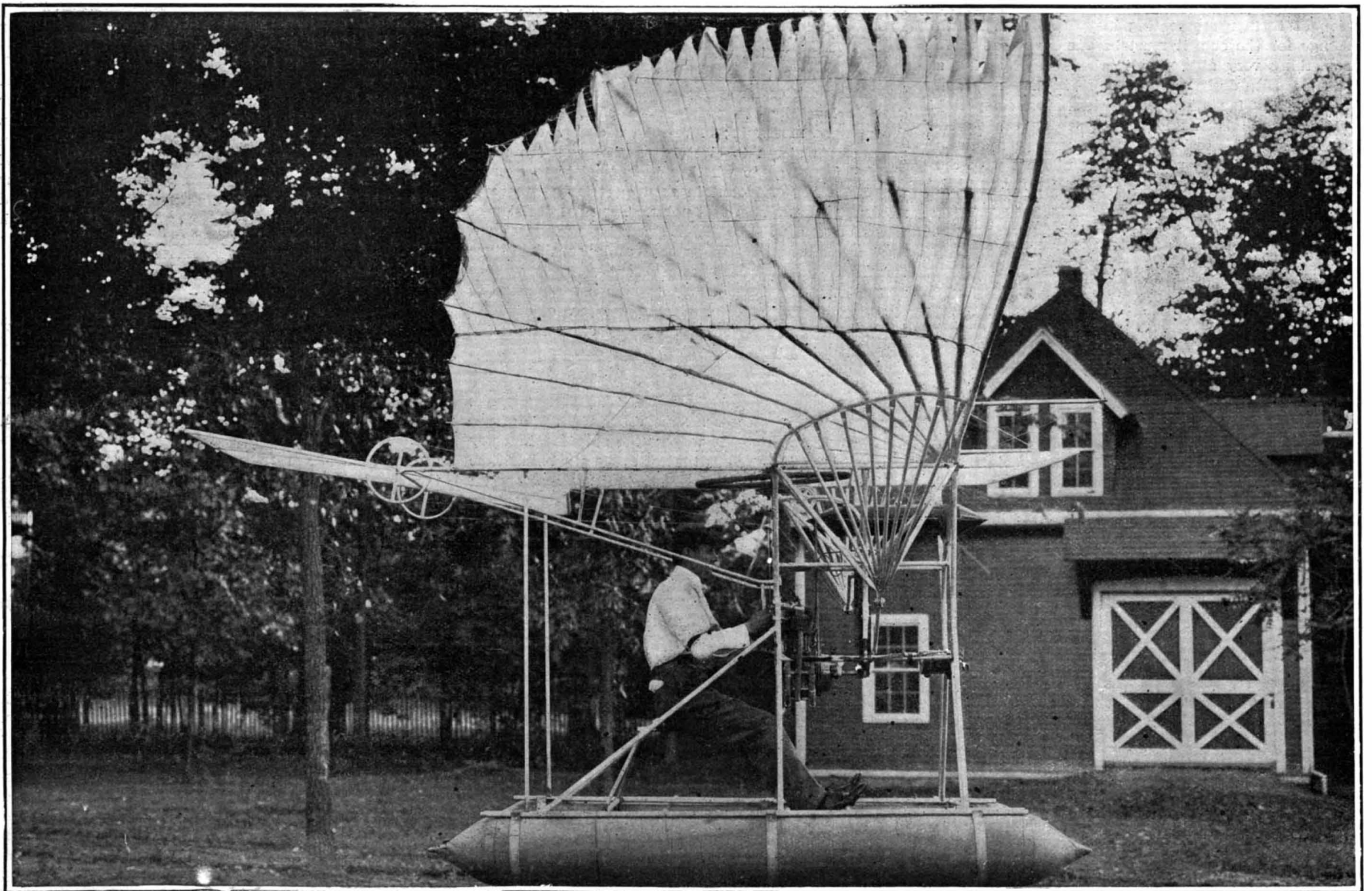
Side View of the Gammeter Orthopter. Weight, 490 Pounds With Operator and Fuel; Engine Rated at 7 Horse-Power; Speed of Engine, 1,200 Revolutions Per Minute; Speed of Wings, 75 Vibrations Per Minute.
