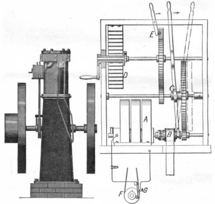
SPARK-PRODUCING MECHANISM FOR EXPLOSION ENGINES.
