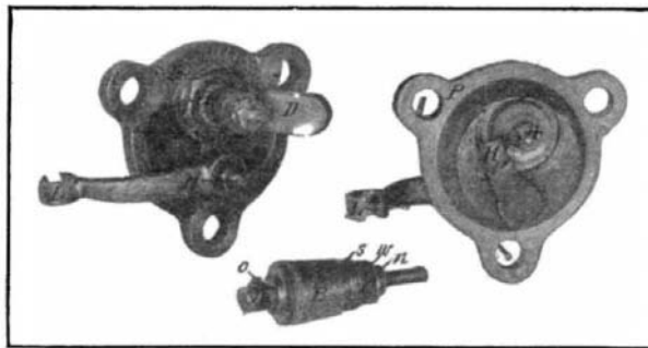
MAKE-AND-BREAK IGNITER OF THE LOCOMOBILE ENGINE.
