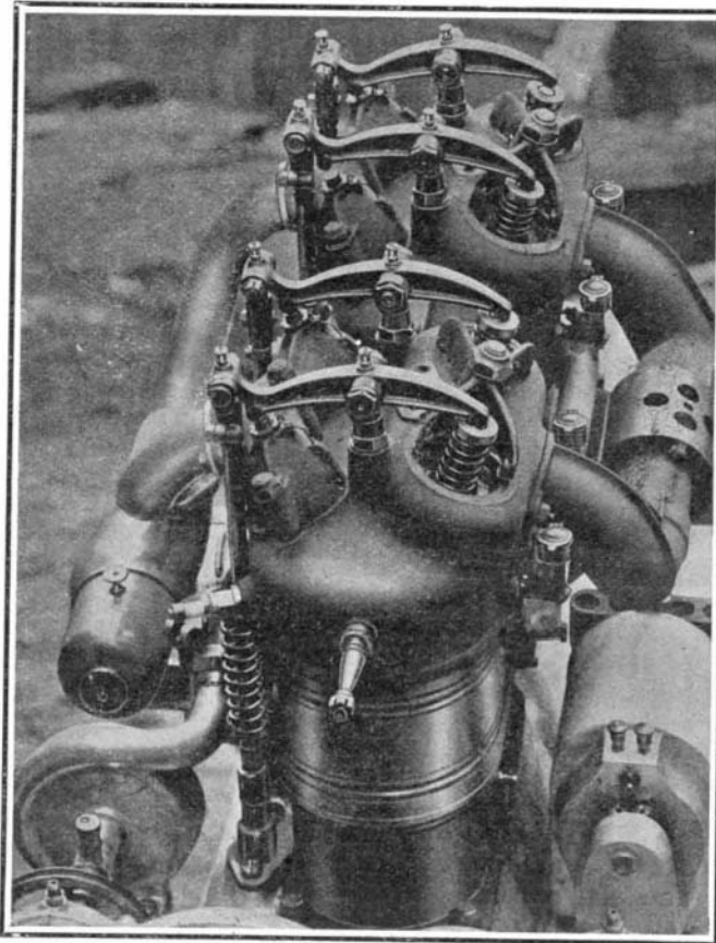
THE 50-HORSE-POWER ENGINE OF THE CAR DE LUXE.
