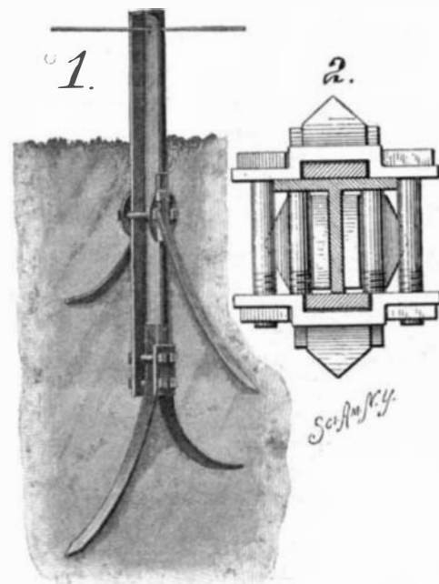
ANCHORING DEVICE FOR POSTS.
