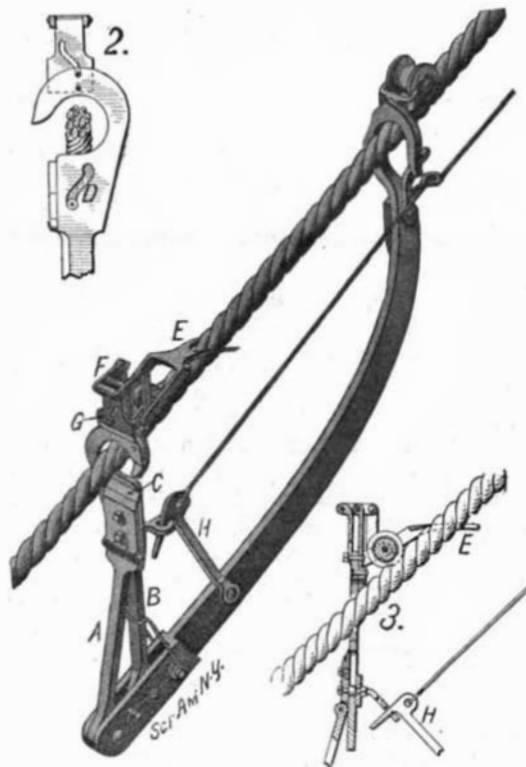
IMPROVED CABLE-CUTTING DEVICE.
