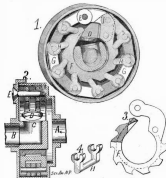
A NOVEL STEAM TRAP.
