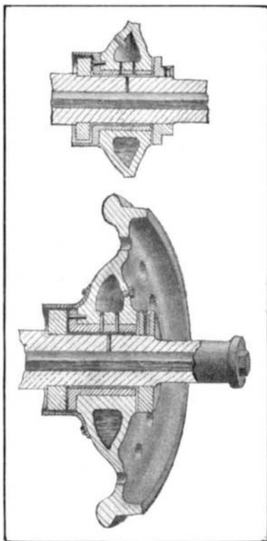
CAR AXLE AND WHEEL.
