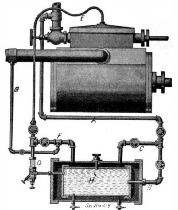
LUBRICATOR FOR STEAM ENGINE CYLINDERS.
