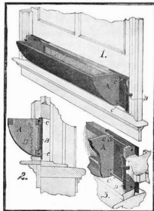
ADJUSTABLE WINDOW VENTILATOR.
