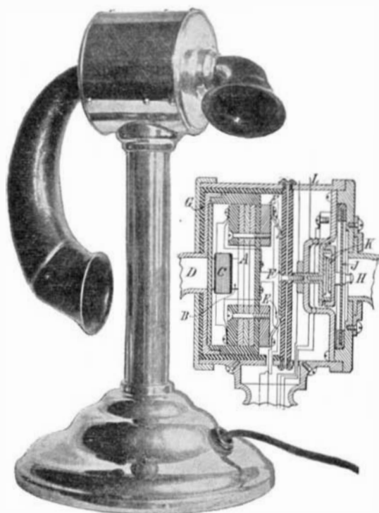
AN IMPROVED TELEPHONE INSTRUMENT.
