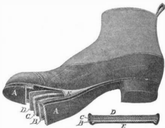
IMPROVED CUSHION SOLE FOR SHOES.
