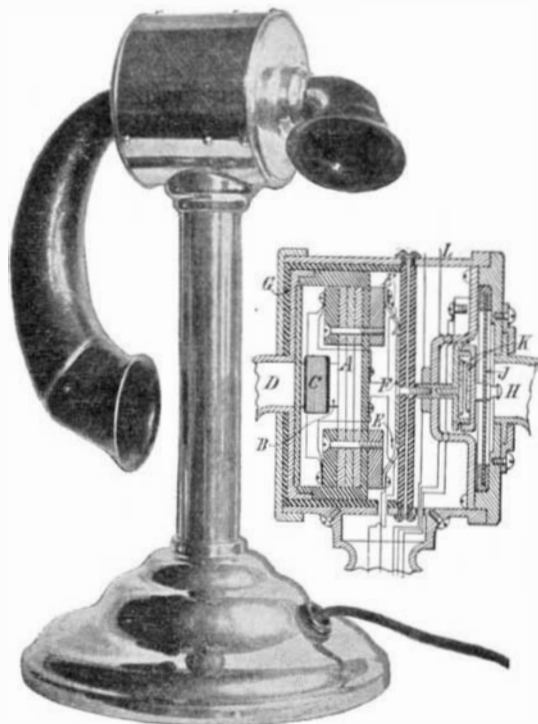
AN IMPROVED TELEPHONE INSTRUMENT.
