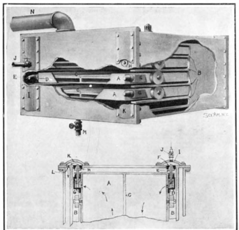
DRYING APPARATUS.
