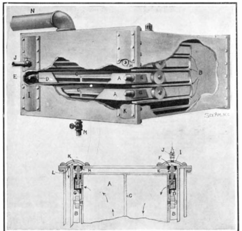
DRYING APPARATUS.
