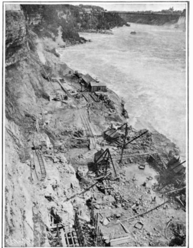
Excavating the Site for the Generating Station at the Foot of the Cliffs.
