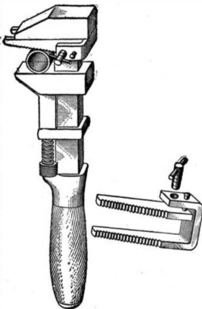
PIPE-GRIPPING ATTACHMENT FOR MONKEY WRENCHES.
