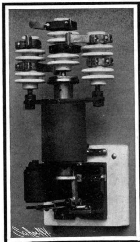
THE SIEMENS-SCHÜCKER AUTOMATIC SWITCH FOR TRANSFORMERS.
