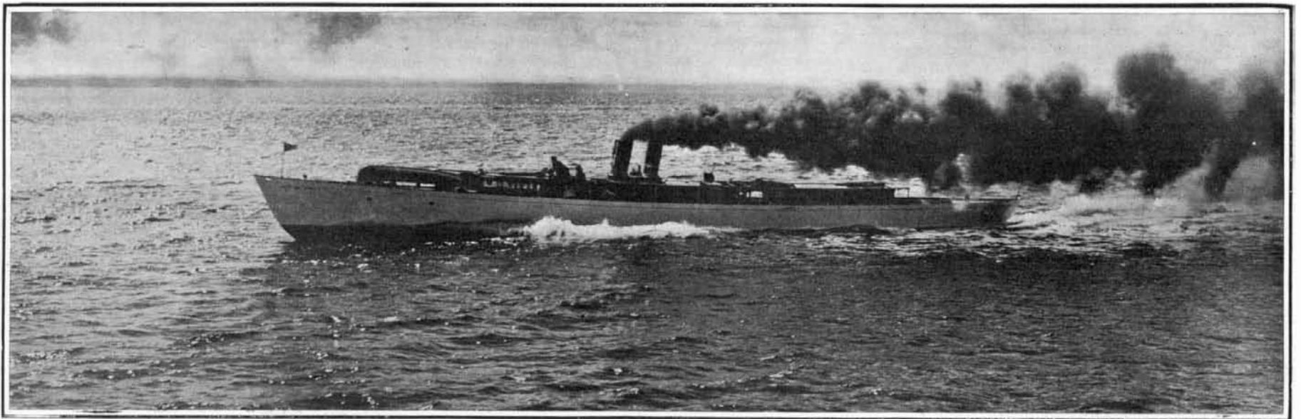
"Niagara IV." Length, 111 Feet. Beam, 12.2 Feet. Draft, 4.2 Feet. Motive Power, Reciprocating Engines. Time Over Course, 1 Hour 56 Min. 3 Sec.
