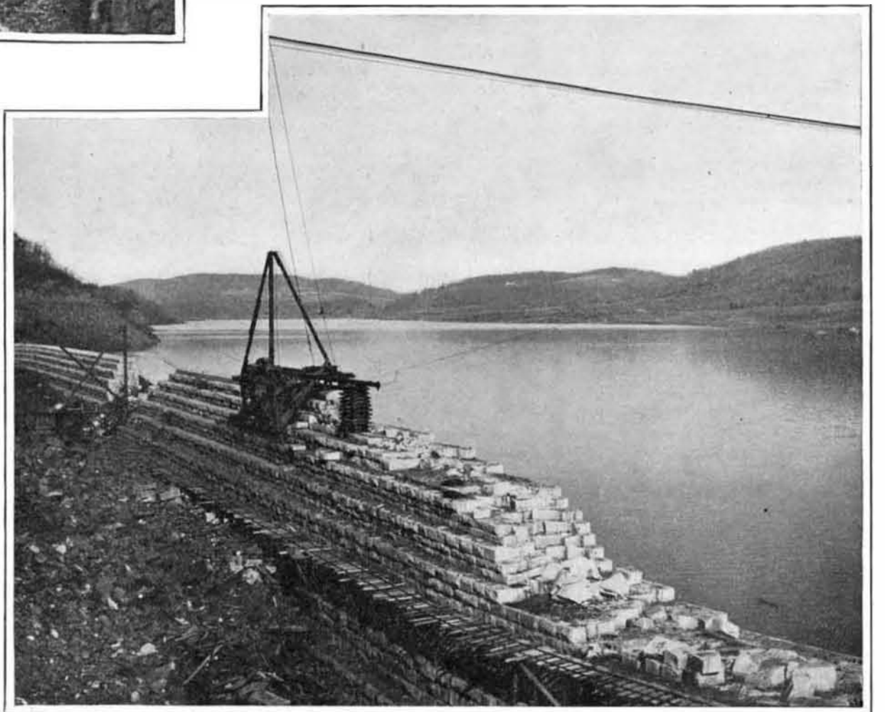
Croton Lake at its Broadest Point ; 20 Miles Long and Holding 30,000,000,000 Gallons.
