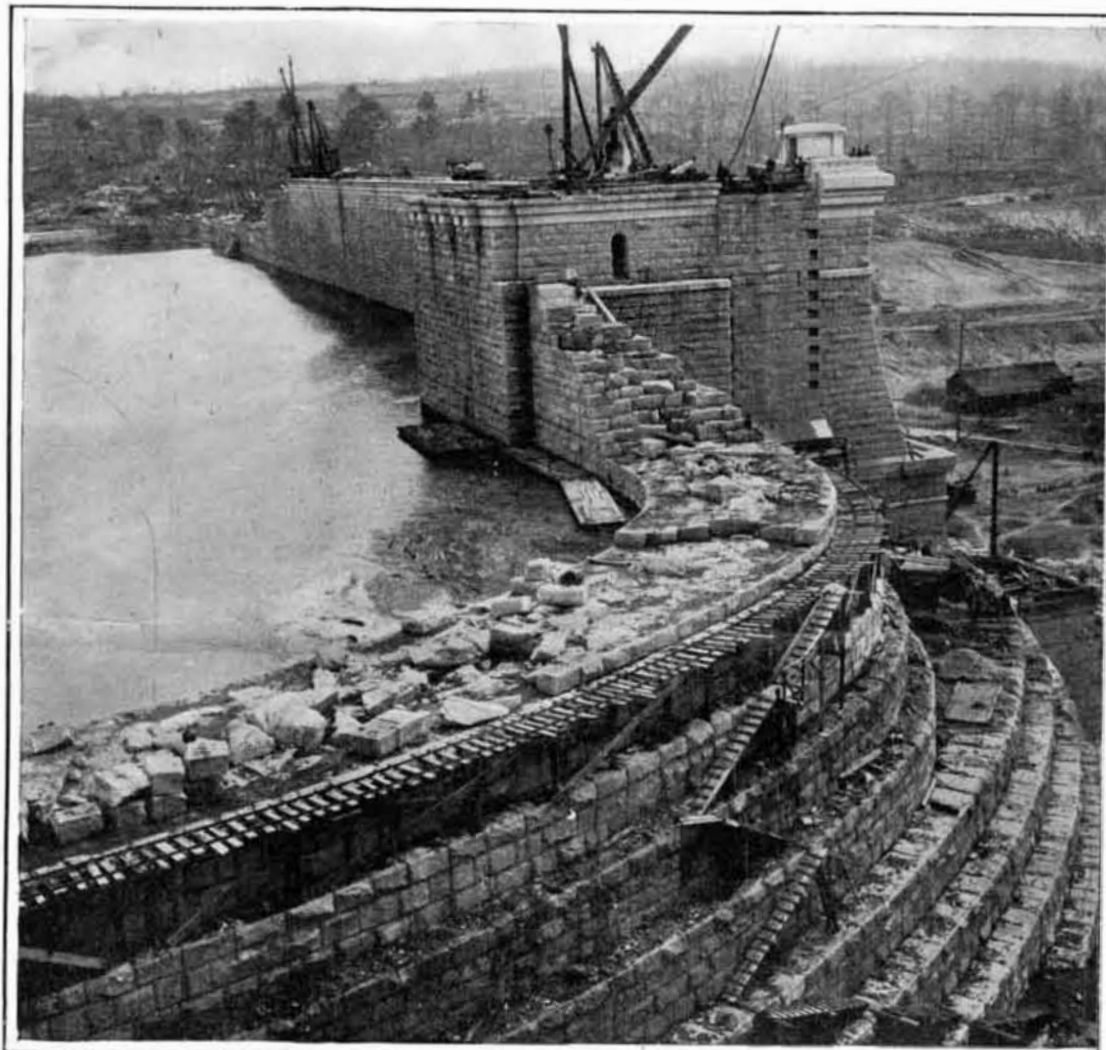
Difference of level between the water within the dam and the river at its toe is 120 feet. All t Looking Down the Croton Valley from
