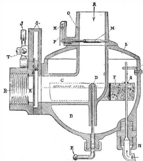
SCHEBLER AUTOMATIC CARBURETER FOR GASOLINE ENGINES.
