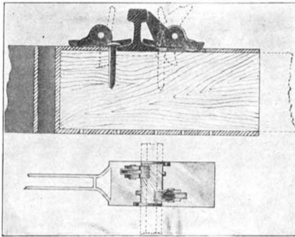
METAL CROSS TIE FOR RAILROADS.
