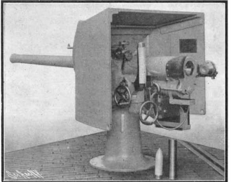
Armstrong 3-Inch Naval Gun, as Mounted on Japanese Ships.
