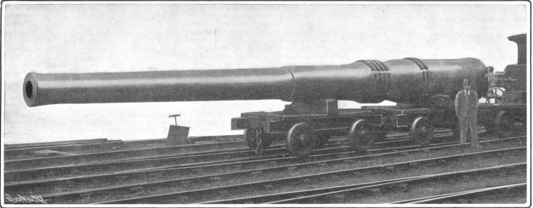
Length, 40 calibers. Caliber, 12 inches. Weight of shell, 850 pounds. Weight of gun, 49 tons. Muzzle velocity, 2,423 foot-seconds. Muzzle energy, 34,600 foot-tons. The Standard Battleship 12-Inch Wire-Wound Gun.
