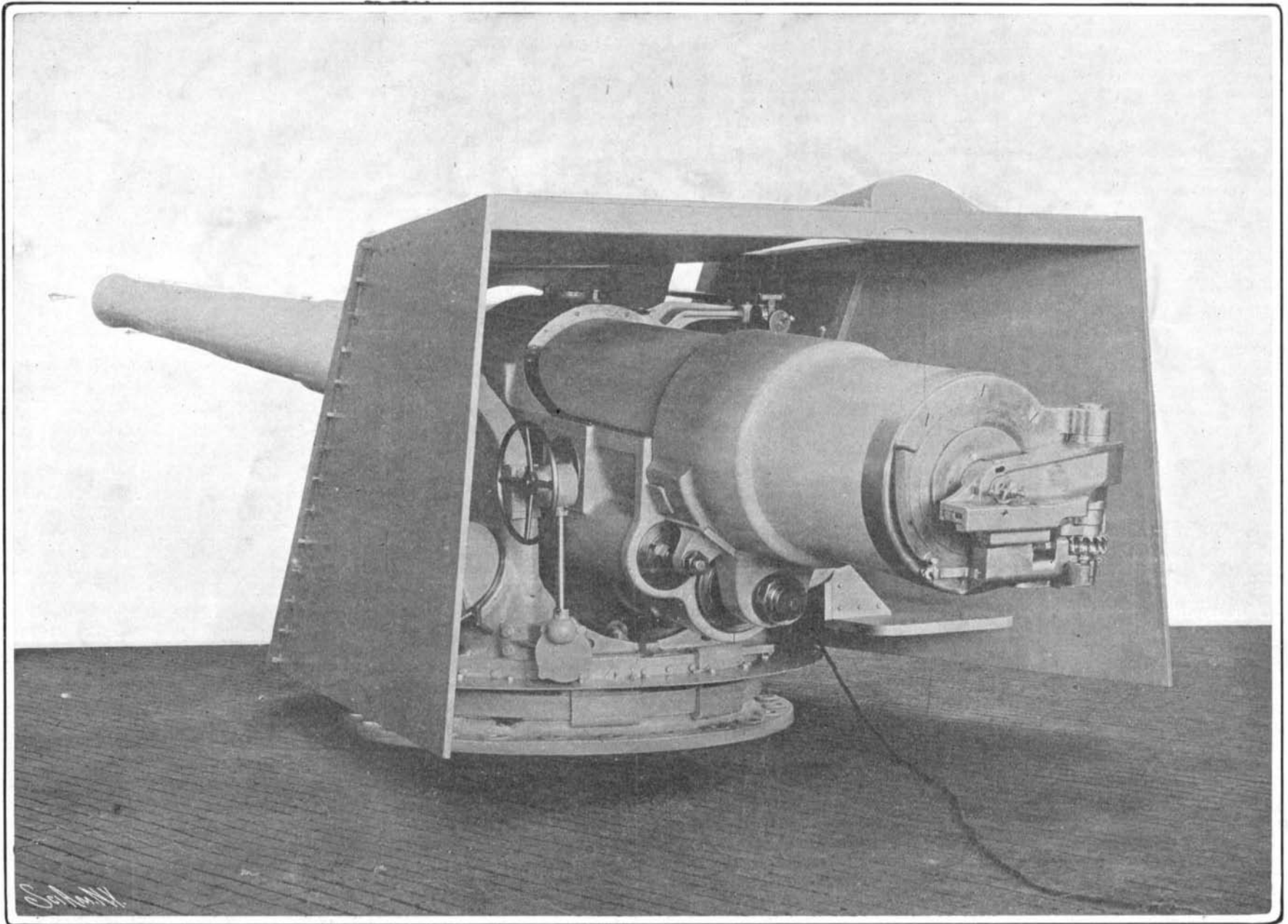
Caliber, 8 inches. Length, 40 calibers. Weight of shell, 250 pounds. Weight of gun, 15¼ tons. Muzzle velocity, 2,068 foot-seconds. Muzzle energy, 7,413 foot-tons. The Standard 8-Inch Cruiser Wire Wound Gun at Present Mounted on Japanese Cruisers.
