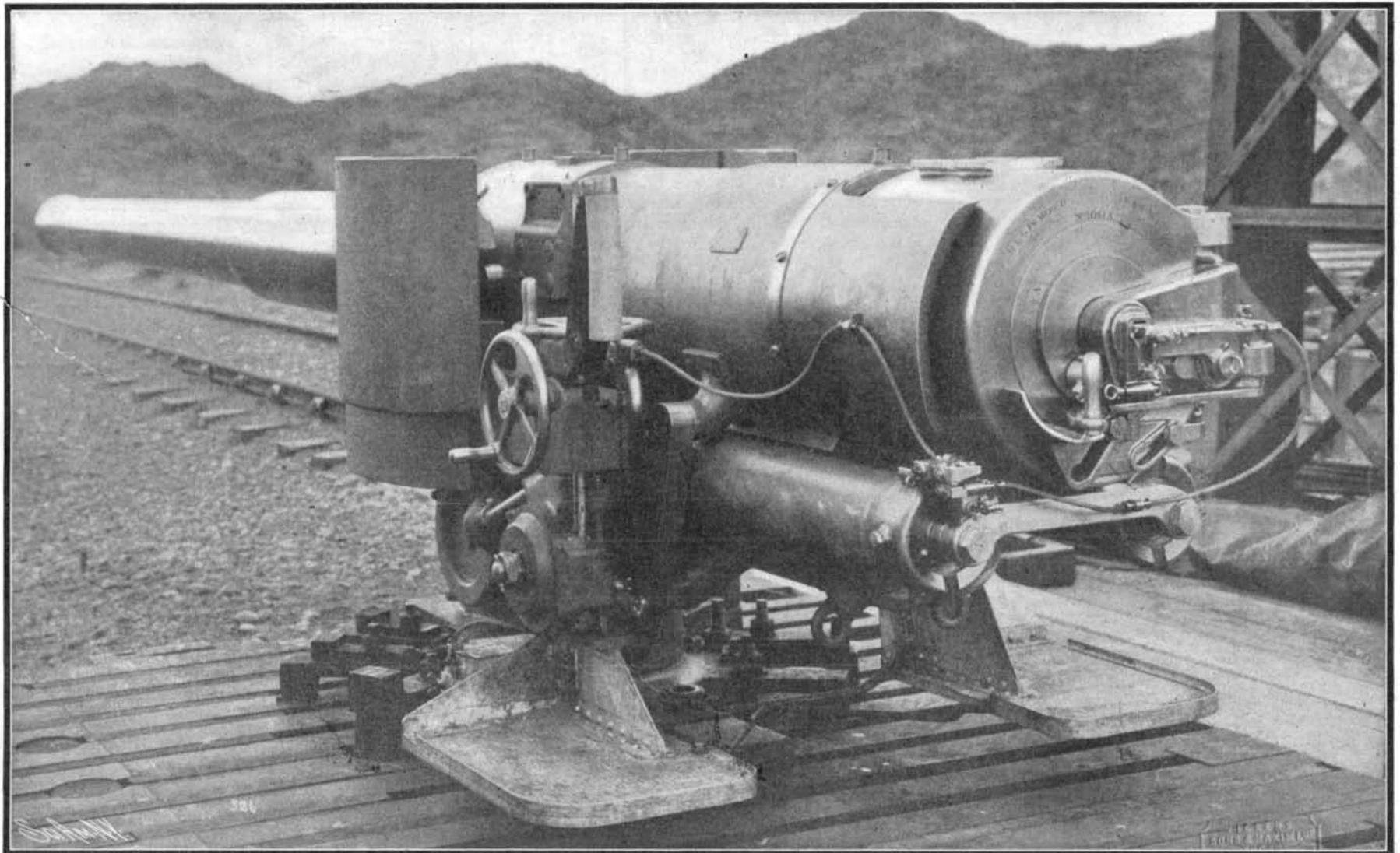
New Vickers-Maxim 6-Inch Gun to be Mounted on the New 16,000-Ton Battleship Recently Ordered by Japan. Velocity at Muzzle, 3,000 Foot-Seconds; Energy, 6,240 Foot-Tons. THE GUNS OF THE JAPANESE NAVY.—[See page 11.]
