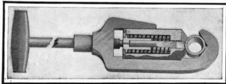
TOOL FOR CUTTING PIPES OR BARS.
