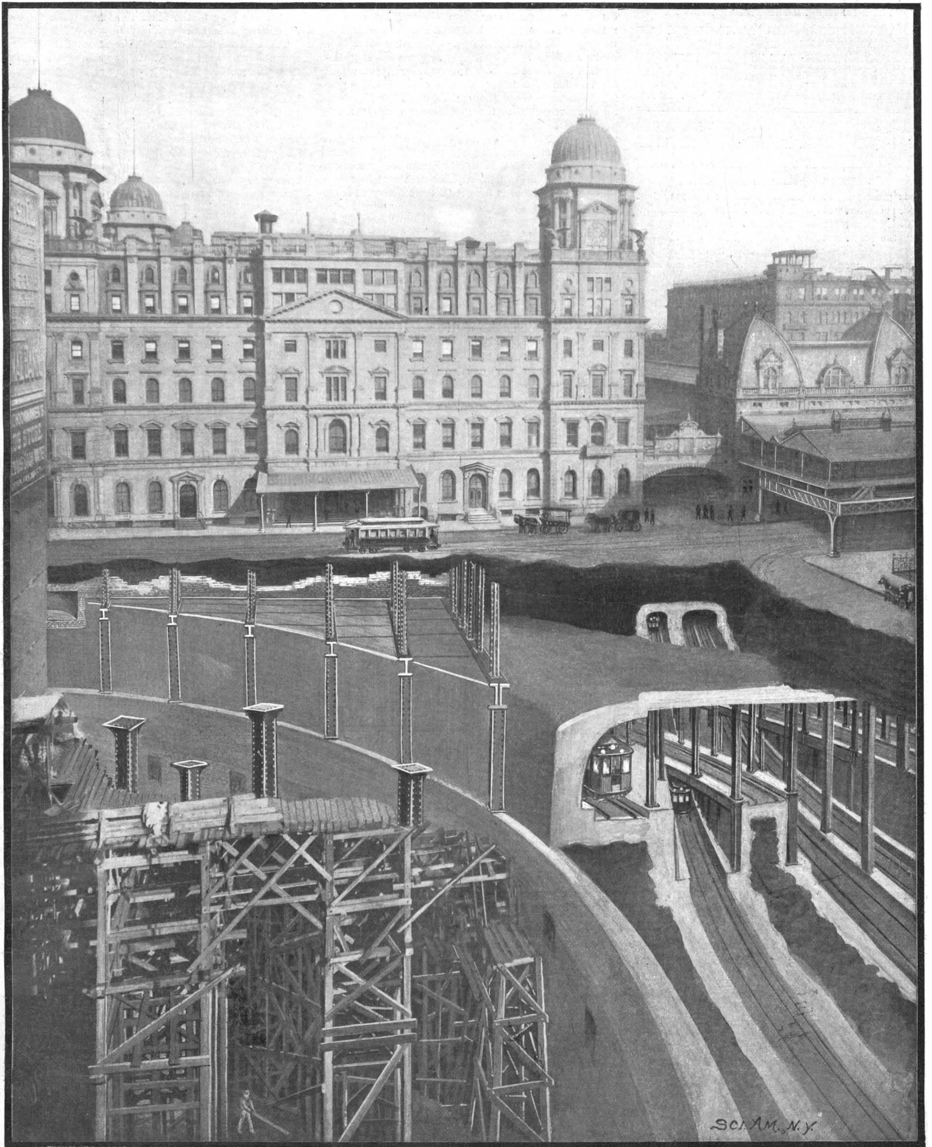
GRAND CENTRAL STATION IMPROVEMENTS AND TRACK CONNECTION WITH THE RAPID TRANSIT SUBWAY.—[See page 39.]
