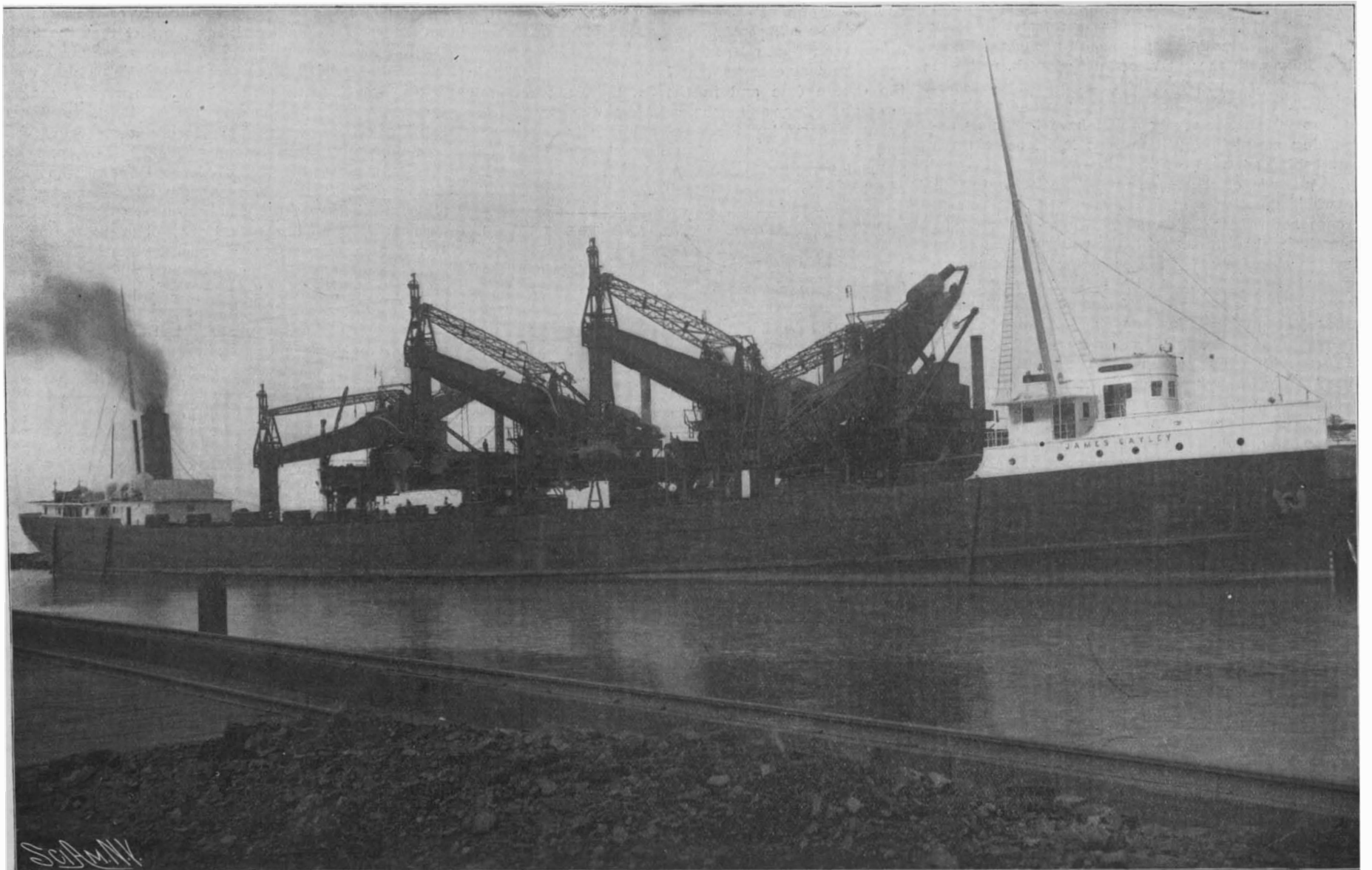
Ore-Unloaders at Work on the Cargo of an Ore-Carrying Steamer.
