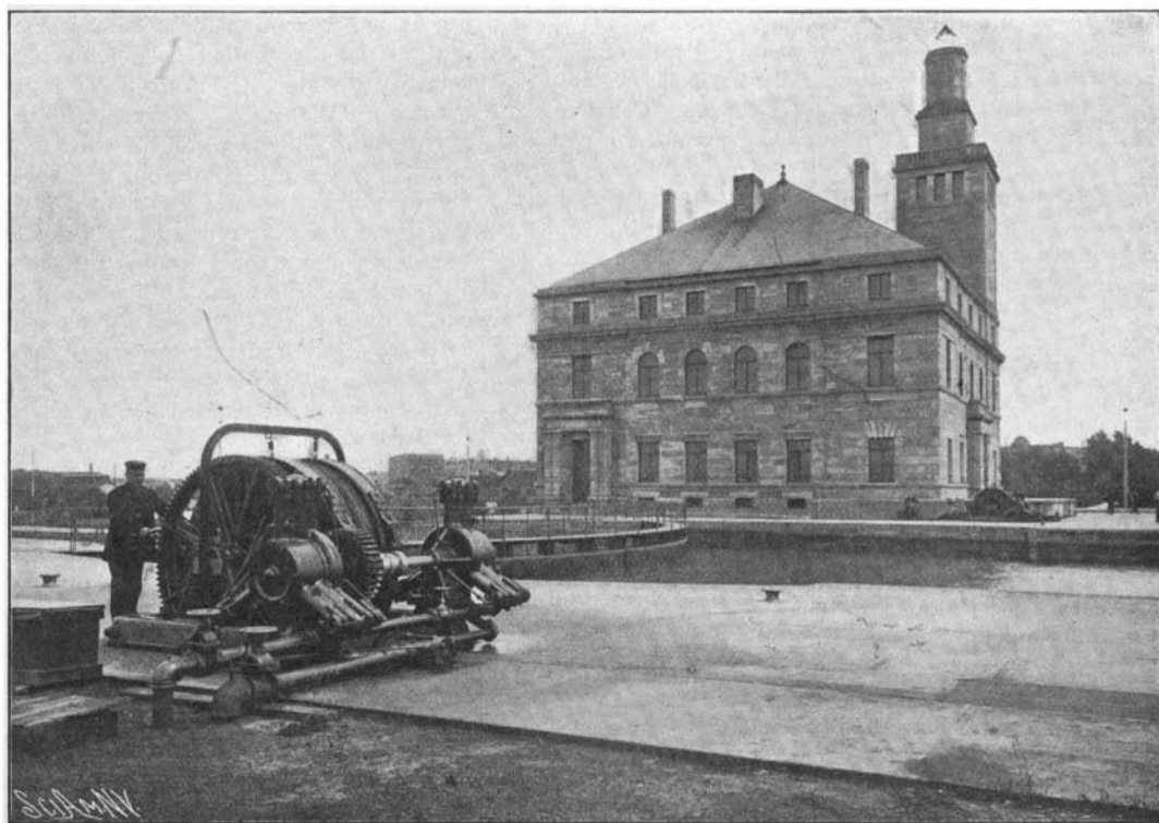
GATE-OPERATING MECHANISM AT SAULT STE. MARIE.
