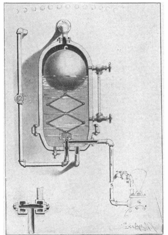
WATER REGULATOR FOR STEAM BOILERS.
