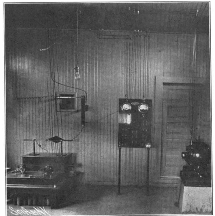
INTERIOR OF THE SANTA CATALINA WIRELESS TELEGRAPH PLANT.
