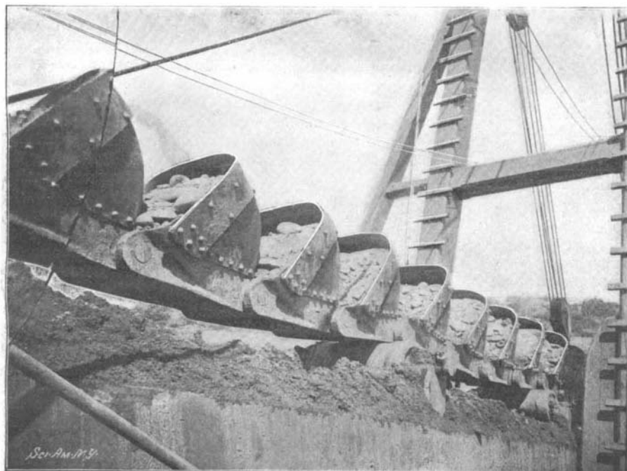
A CONTINUOUS BUCKET DREDGER.
