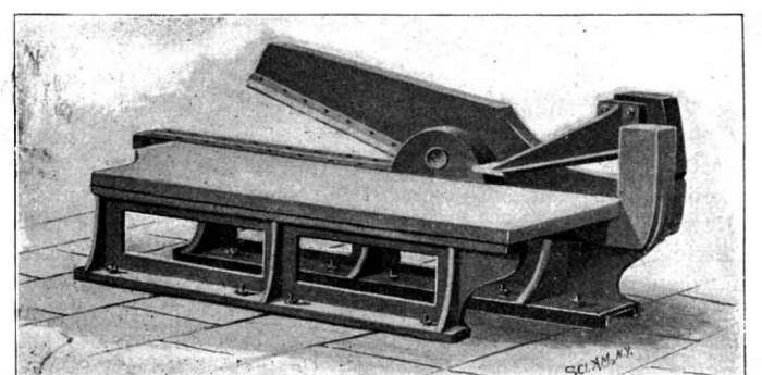
Doubling Shears in Which Plates are Folded.
