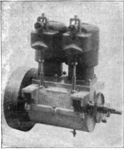
16 H. P. motor, weight 220 lbs. MOHLER & DE GRESS, Long Island City, N. Y.
