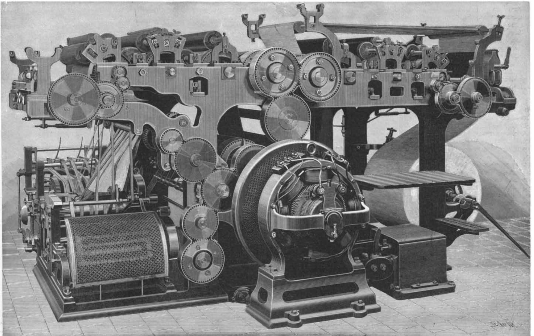
Motor Direct-Connected to a German High-Speed Rotary Press.
