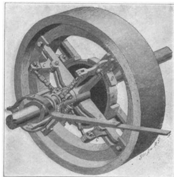
POWERFUL FRICION CLUTCH PULLEY.
