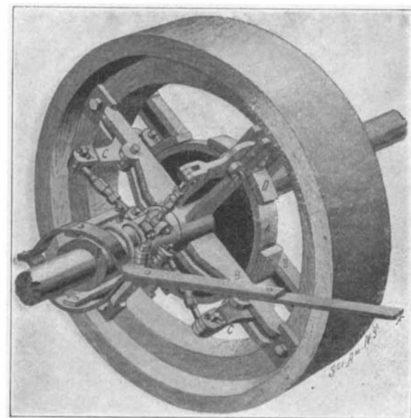
POWERFUL FRICTION CLUTCH PULLEY.
