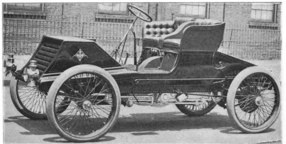
Fig. 4.—A Typical American High Power Racer—Winton 40 Horse Power Machine.
