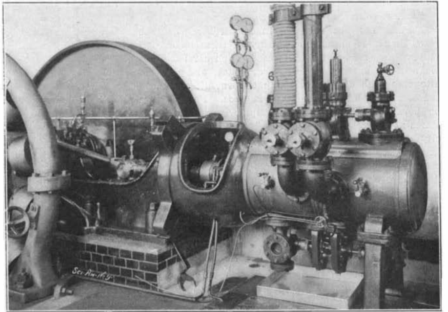
Waste-Heat Engine at Technical High School.
