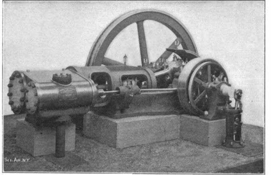
Waste-Heat Engine, Berlin Electrical Power Station.
