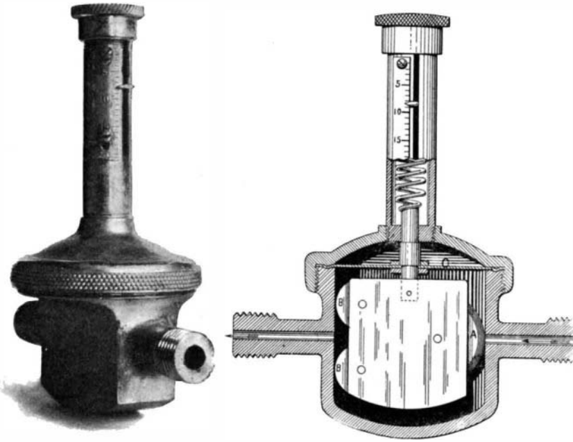
AN AUTOMATIC REDUCING VALVE.
