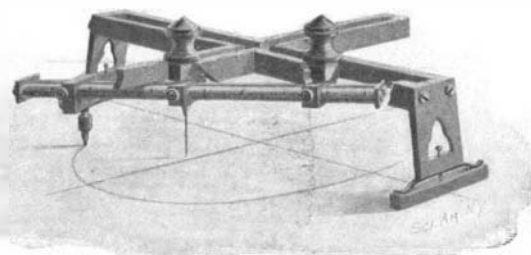
AN ELLIPSOGRAPH.
