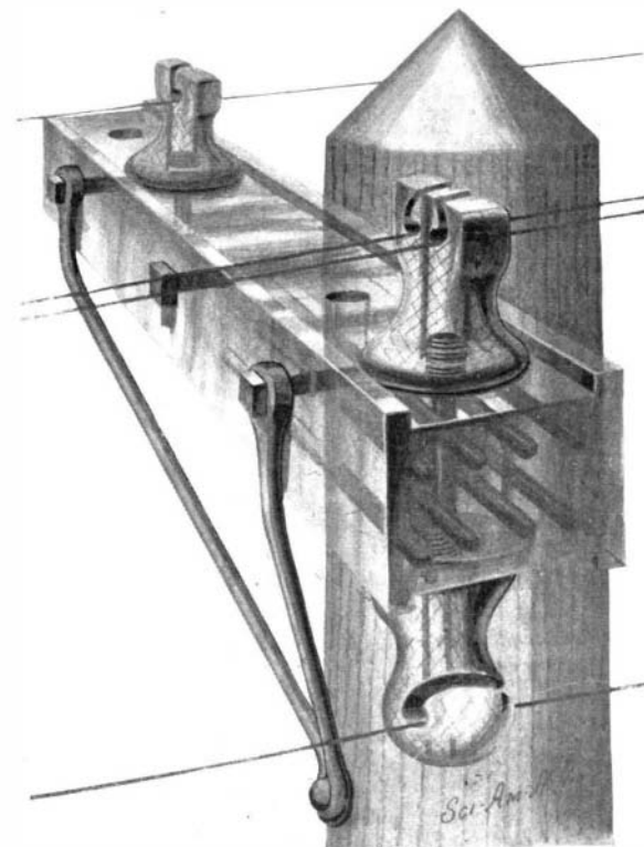
THE WOOLBERT INSULATOR.
