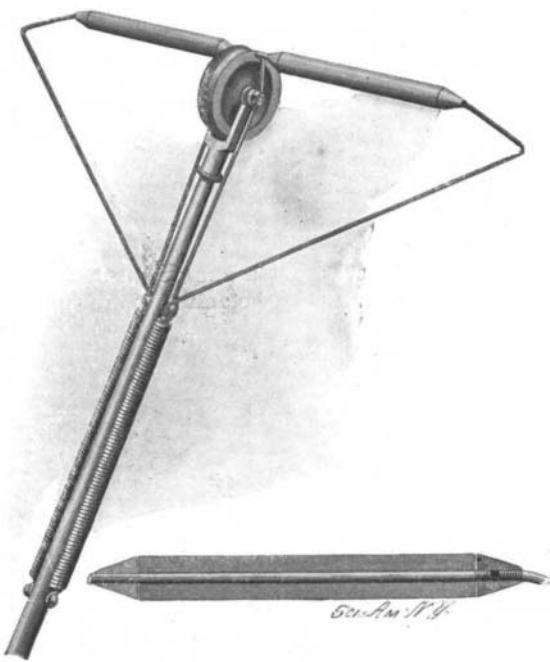
AN IMPROVED TROLLEY-POLE GUARD.
