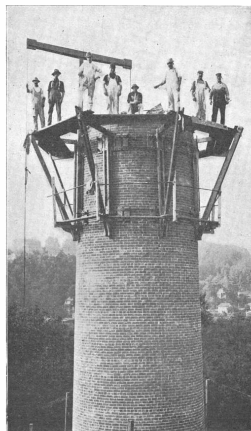
A NEW STAGING FOR BUILDING CHIMNEYS.
