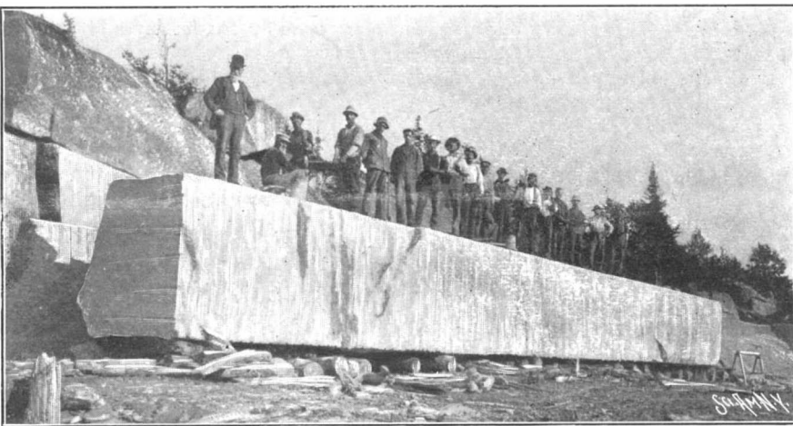
Blank for Column 64 Feet Long, 8 Feet 6 Inches by 7 Feet.
