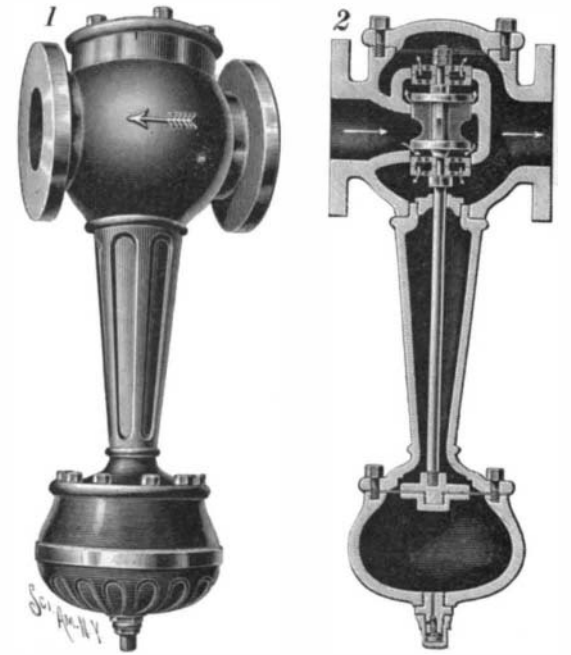
A SIMPLE PRESSURE REGULATOR.
