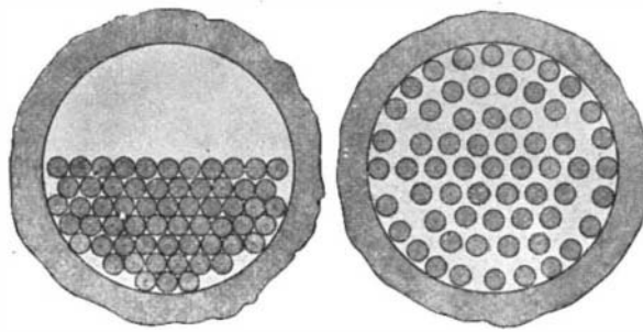
FIG. 1.—Approximate position of the powder in the gun before ignition. FIG. 2.—Approximate position of the sticks of powder in the gun after firing. Sticks are nearly full length of powder chamber.
