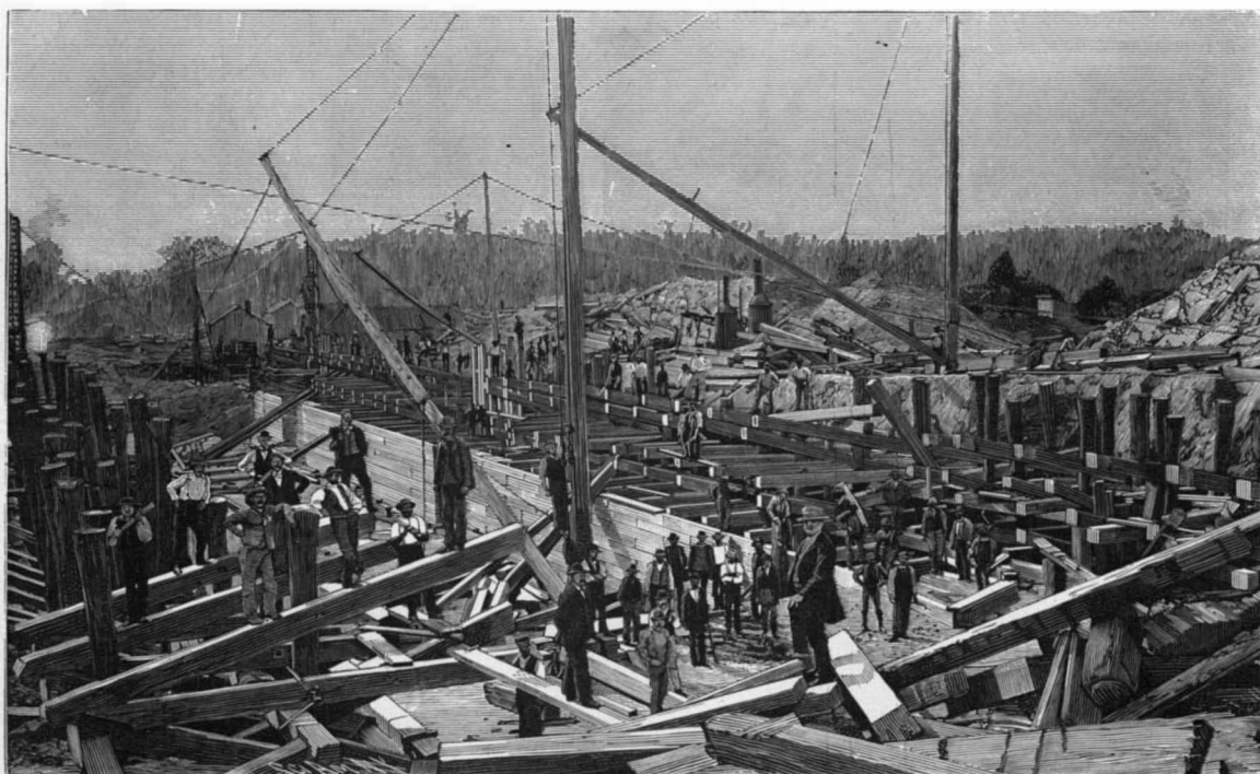
Fig. 3.—CONSTRUCTION OF LOCKS, DISMAL SWAMP CANAL.
