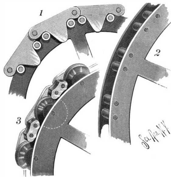
1 and 2. Wizard bicycle chain and sprocket. 3. Brown roller sprocket. THE WIZARD CHAIN AND BROWN SPROCKET.
