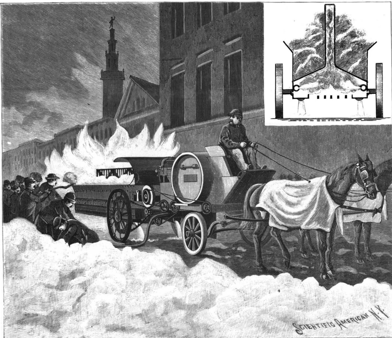
REMOVING SNOW FROM STREETS BY THE PROCESS OF MELTING.
