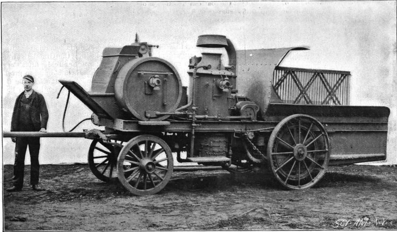
SNOW MELTING MACHINE NOW BEING USED IN THE STREETS OF NEW YORK.
