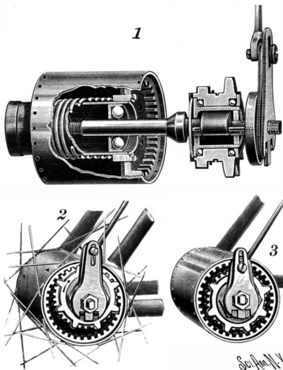
1. Sectional view of gear. 2. Gear in low speed position. 3. Gear in high speed position. THE JOHNSTON TWO SPEED GEAR.
