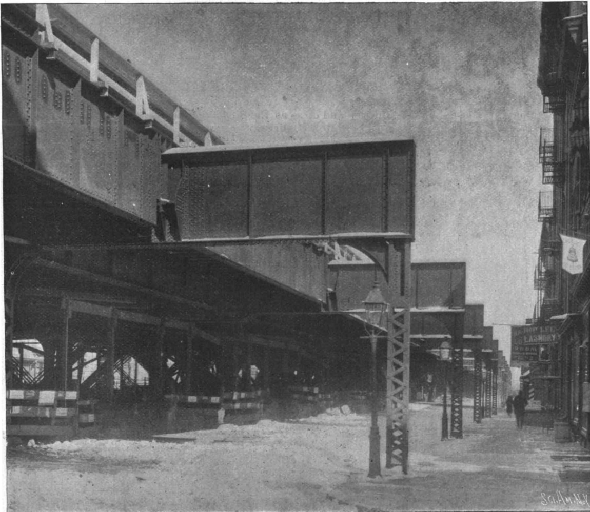
AUXILIARY GIRDERS FOR CARRYING LOCAL TRACKS AT ONE HUNDRED AND TWENTY-FIFTH STREET STATION. THE NEW YORK CENTRAL FOUR TRACK STEEL VIADUCT NEW YORK.
