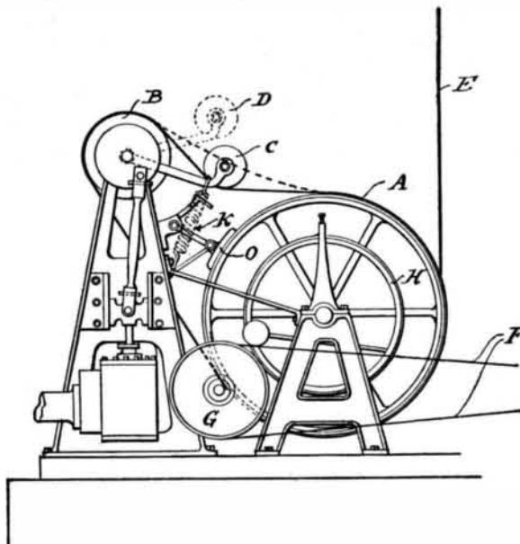
SKETCH OF POST OFFICE ELEVATOR HOISTING ENGINE.
