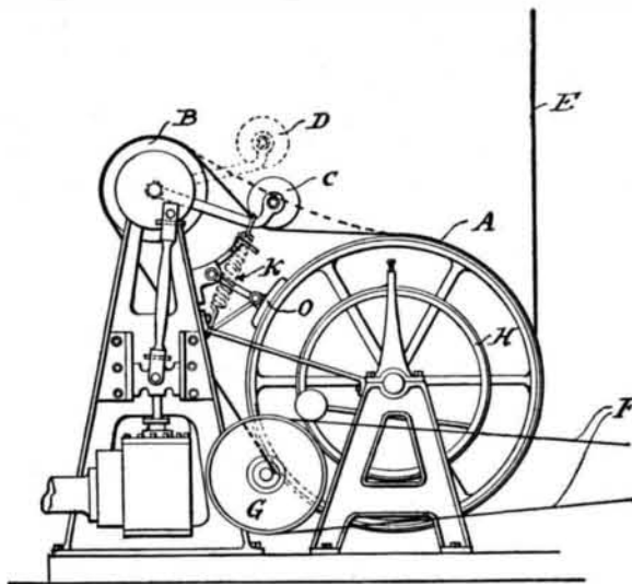
SKETCH OF POST OFFICE ELEVATOR HOISTING ENGINE.
