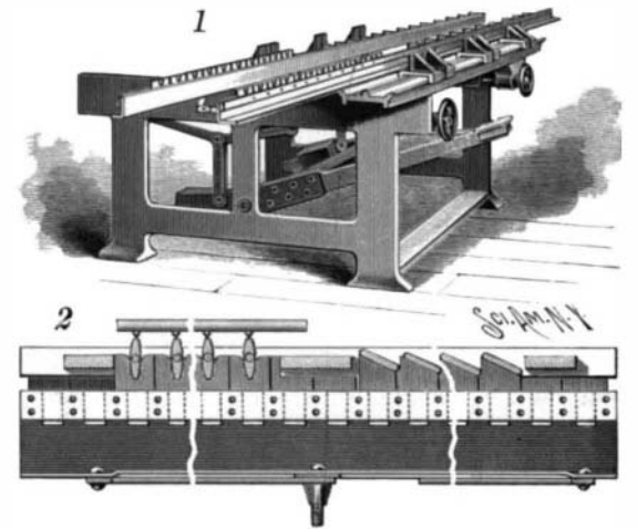
PARKS AND NELSON'S BLIND SLATTING MACHINE.
