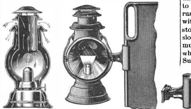
THE "DIETZ" TUBULAR DRIVING LAMP.
